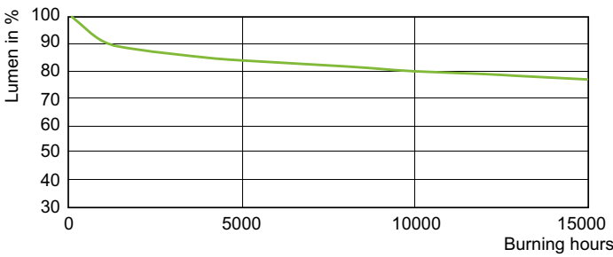
Lumen Maintenance Diagram - MASTERC CDM-T Elite 70W/942 G12 1CT
